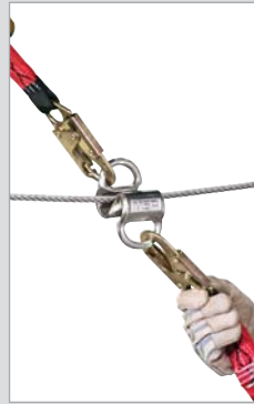
Gravity® Horizontal Lifeline Bypass Shuttles
