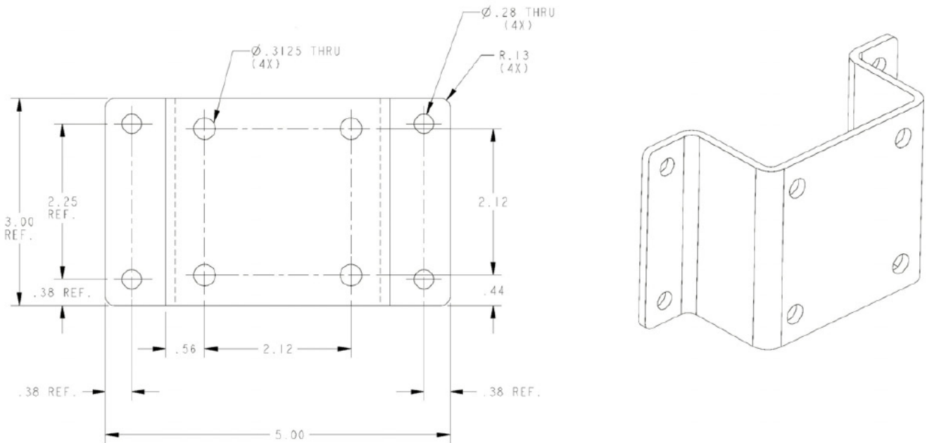
Figure 6 Mounting bracket for Stainless Steel Junction Box
