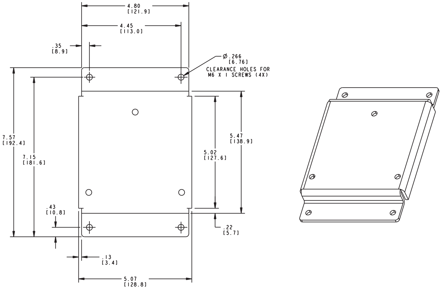
Figure 6 Mounting bracket for Stainless Steel Junction Box
